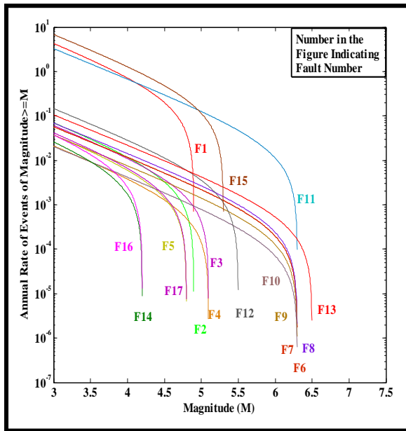
Figure 4: Deaggregation of Seismic Sources Near Sikaser Dam
