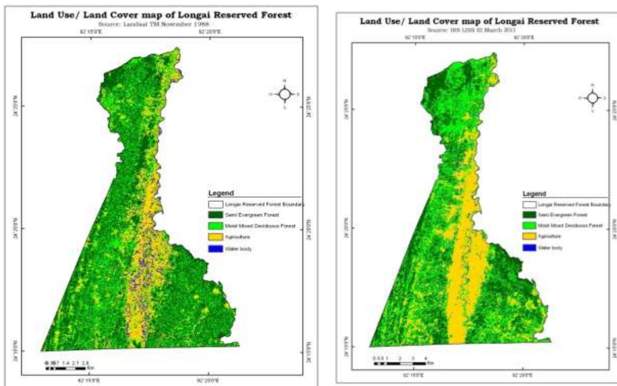
Figure.2 Comparative map showing Land Use/land Cover changes in Longai Reserve Forest ( From 1988 to 2011)
